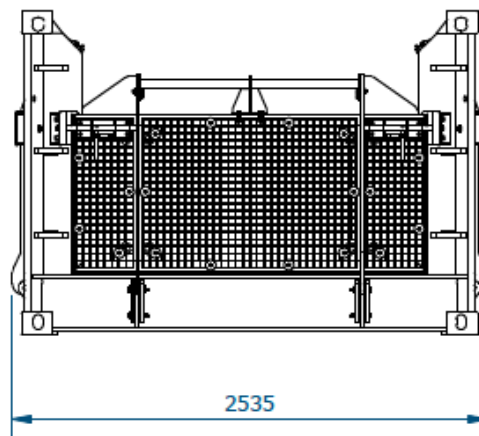
VIEW2 ( 1 : 40 )
